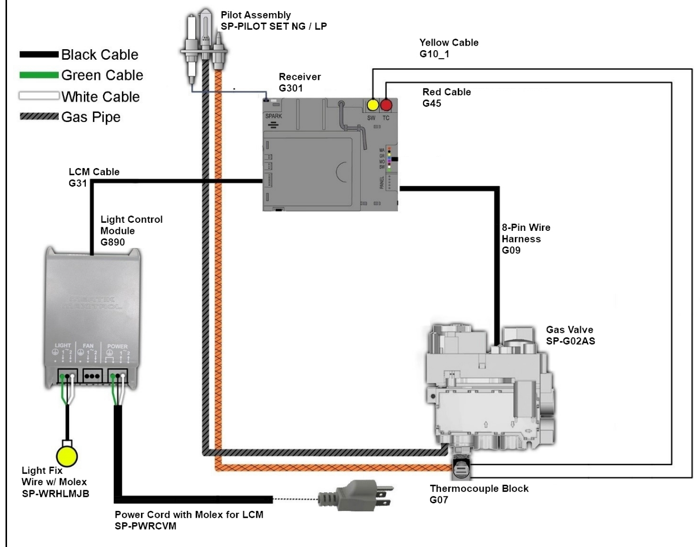
Wiring Diagram: Screen Fireplace with Interior Lighting
