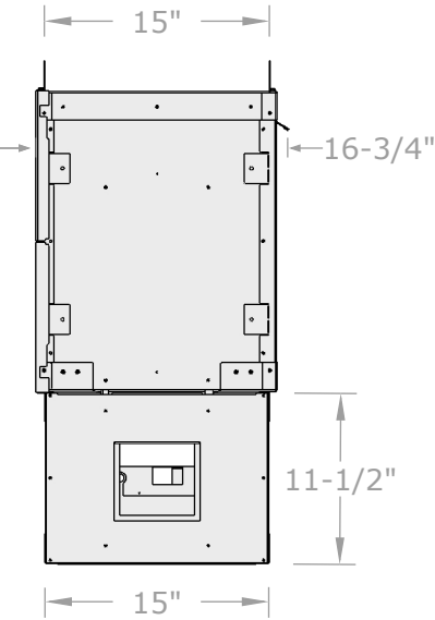
BACK VIEW (LEFT) SCALE 1:14
