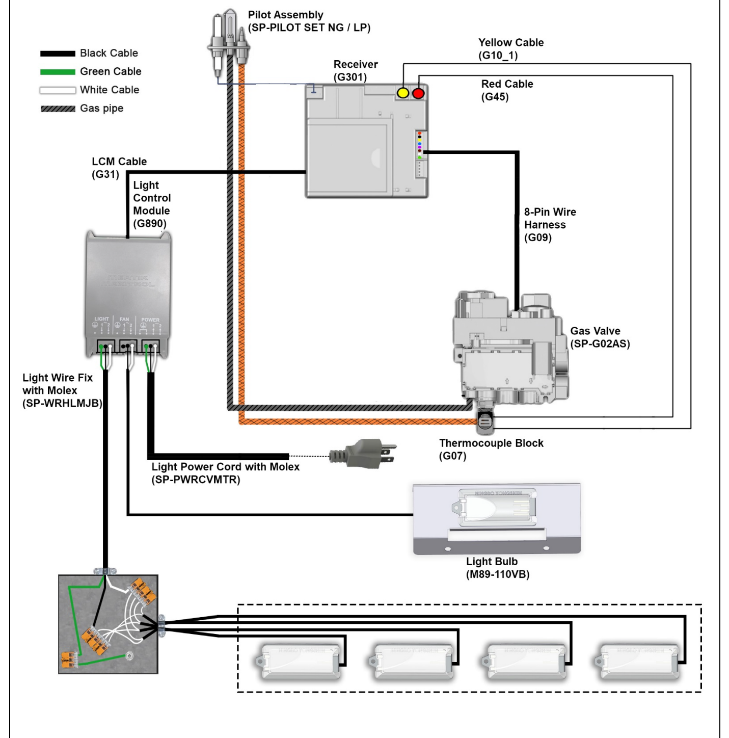
Wiring Diagram: Screen Fireplace with Interior Lighting
