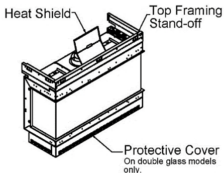
Zero-Clearance Stand-Offs (Isometric View)
