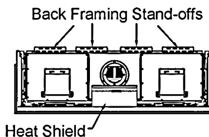
Zero-Clearance Stand-Offs (Top View)
