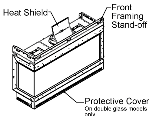
Zero-Clearance Stand-Offs (Isometric View)
