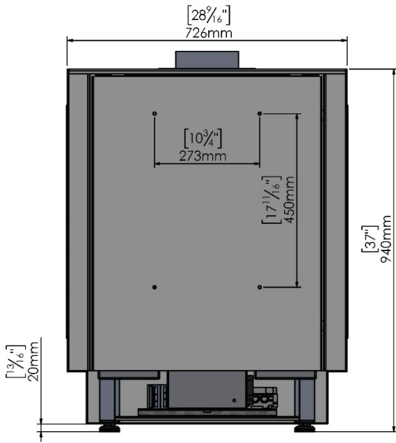
FLOOR-MOUNTED (legs, covered back)
