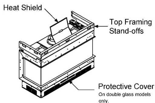
Zero-Clearance Stand-Offs (Isometric View)
