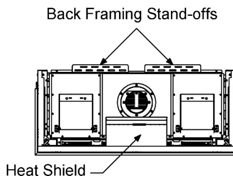
Zero-Clearance Stand-Offs (Top View)
