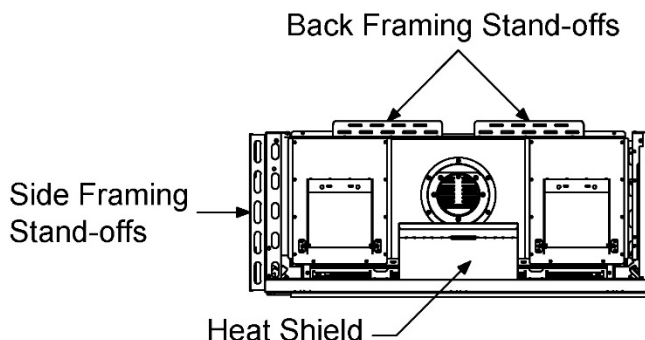
Zero-Clearance Stand-Offs (Top View)
