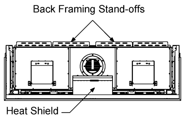
Zero-Clearance Stand-Offs (Top View)
