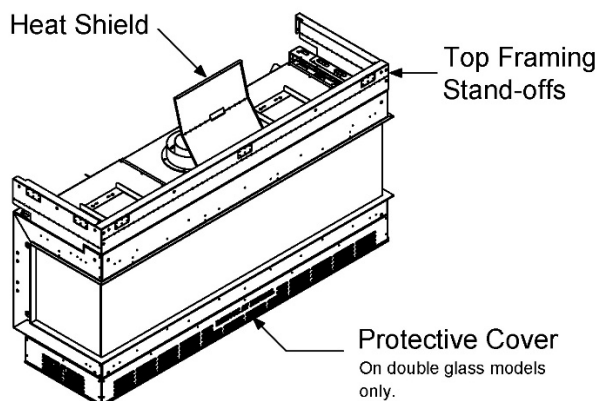
Zero-Clearance Stand-Offs (Isometric View)
