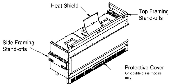
Zero-Clearance Stand-Offs (Isometric View)
