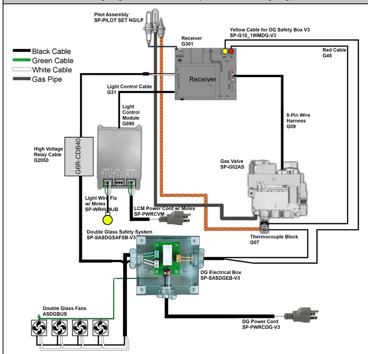
Wiring Diagram: Double Glass Fireplace with Interior Lighting
