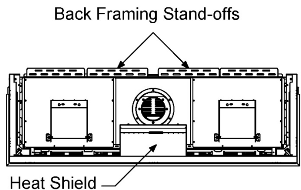
Zero-Clearance Stand-Offs (Top View)
