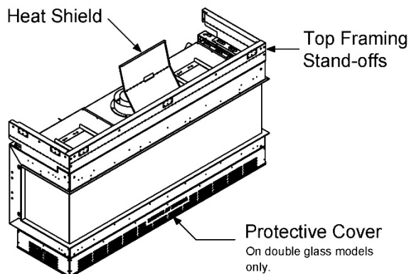
Zero-Clearance Stand-Offs (Isometric View)
