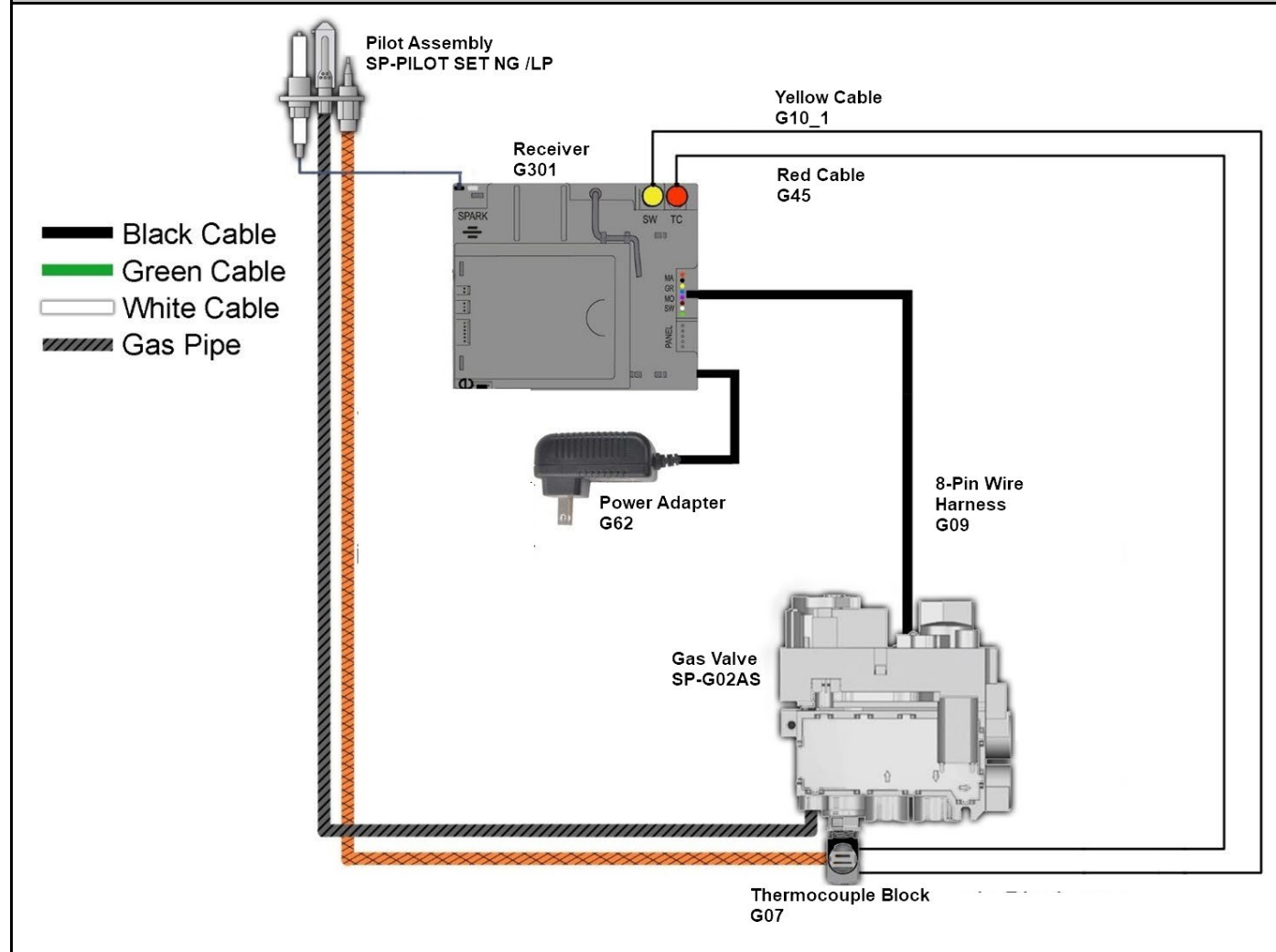
Wiring Diagram: Screen Fireplace
