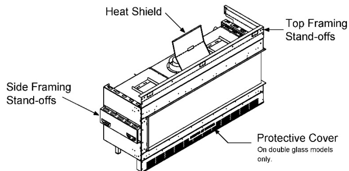
Zero-Clearance Stand-Offs (Isometric View)
