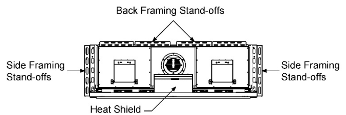
Zero-Clearance Stand-Offs (Top View)
