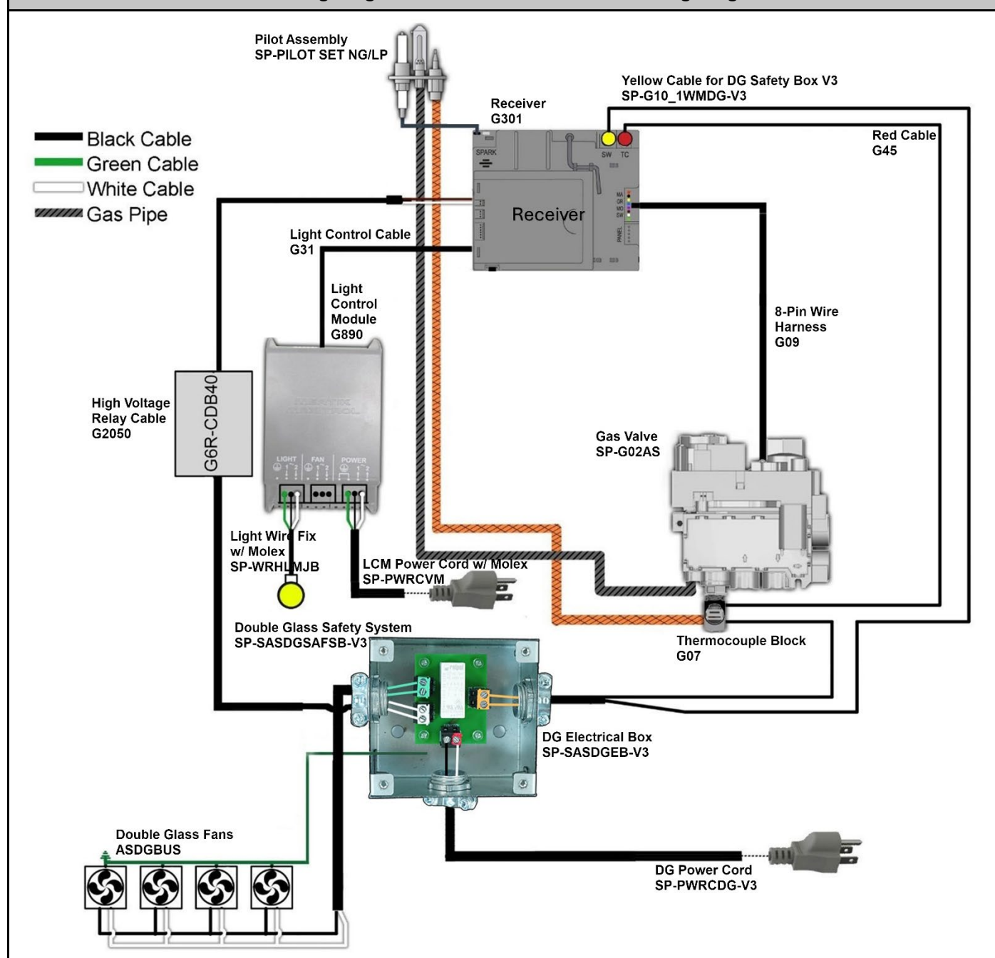
Wiring Diagram: Double Glass with Interior Lighting
