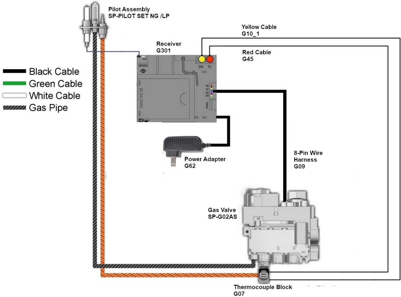
Wiring Diagram: Screen Fireplace
