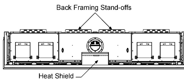
Zero-Clearance Stand-Offs (Top View)
