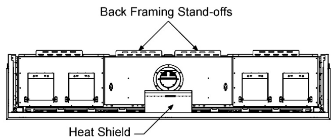
Zero-Clearance Stand-Offs (Top View)
