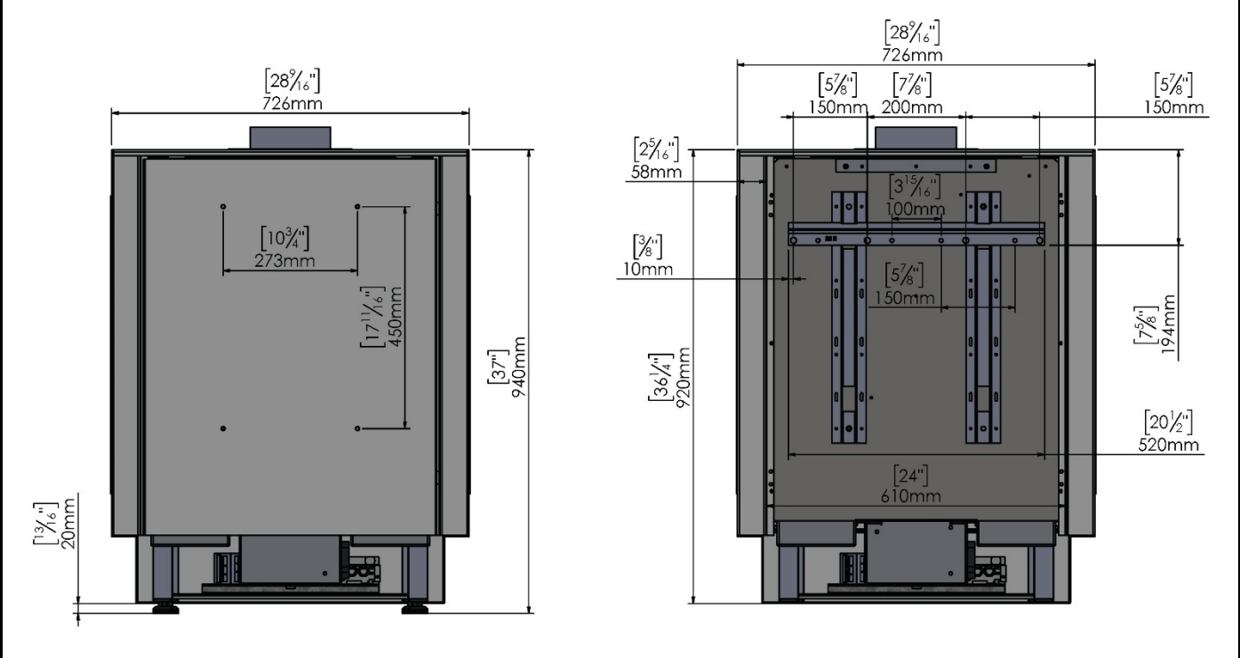
FLOOR-MOUNTED (legs, covered back) WALL-MOUNTED (no legs, exposed mounting attachments on back)
