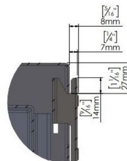
DETAIL F SCALE 1 : 2
