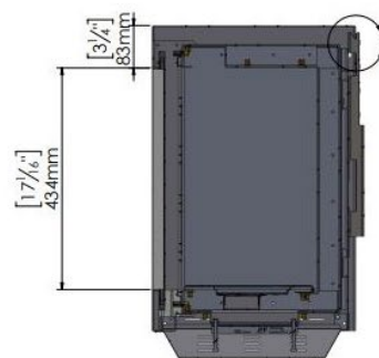
DETAIL F SCALE 1 : 2
