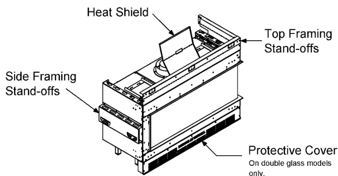
Zero-Clearance Stand-Offs (Isometric View)
