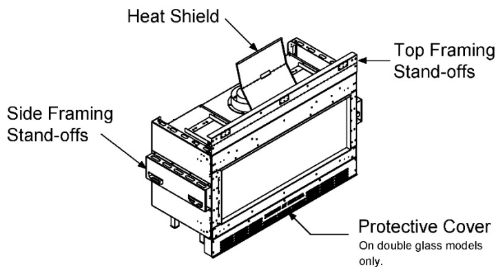
Zero-Clearance Stand-Offs (Isometric View)
