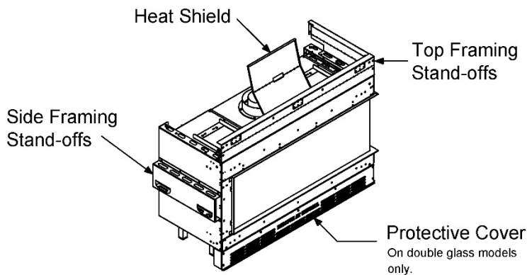
Zero-Clearance Stand-Offs (Isometric View)
