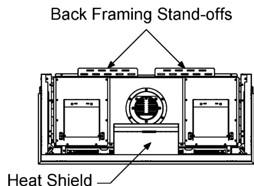
Zero-Clearance Stand-Offs (Top View)
