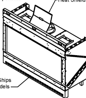
Movable Gas & Electrical Components
