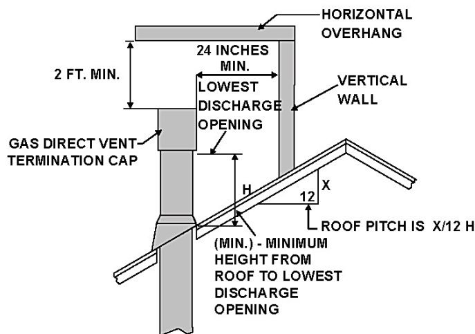
Minimum Height From Roof To Lowest Discharge Opening
