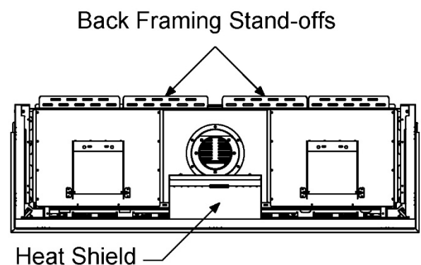
Zero-Clearance Stand-Offs (Top View)
