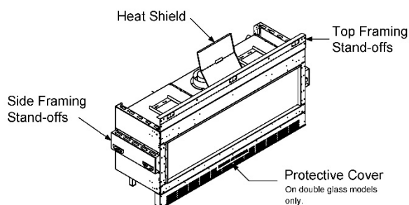
Zero-Clearance Stand-Offs (Isometric View)
