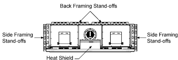
Zero-Clearance Stand-Offs (Top View)
