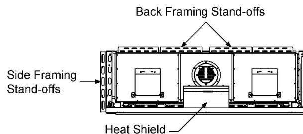
Zero-Clearance Stand-Offs (Top View)
