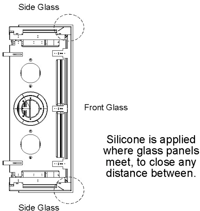
Glass Seal Assembly Diagram
