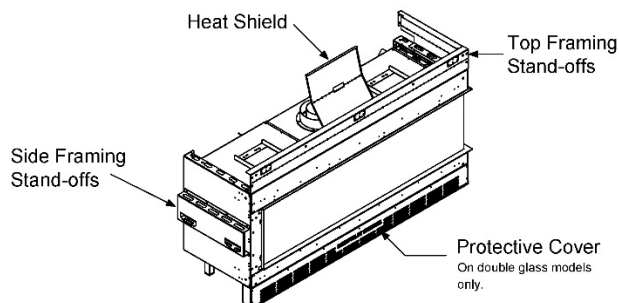
Zero-Clearance Stand-Offs (Isometric View)
