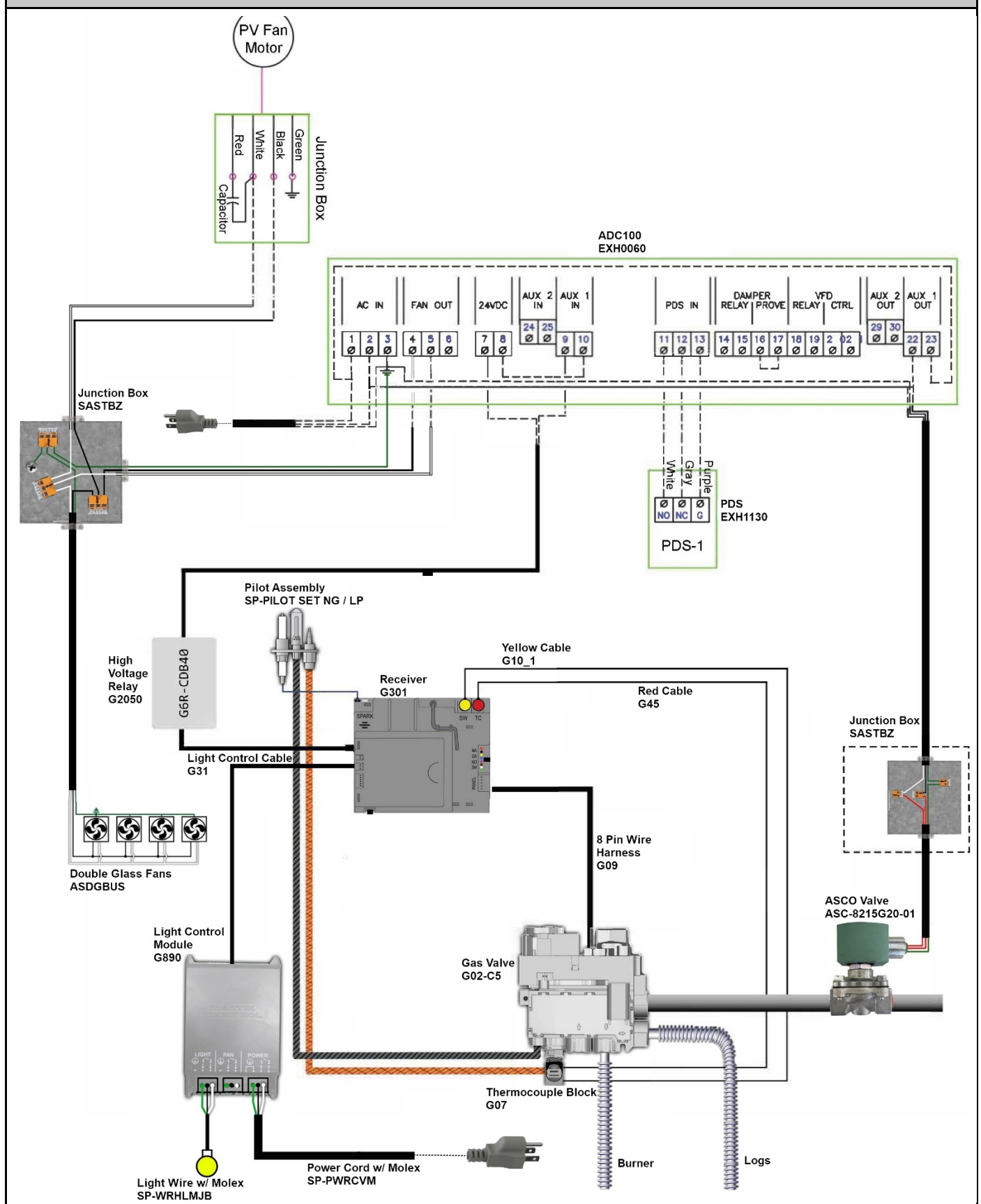
Wiring Diagram: Double Glass Fireplace with Interior Lighting and Enervex Power Vent
