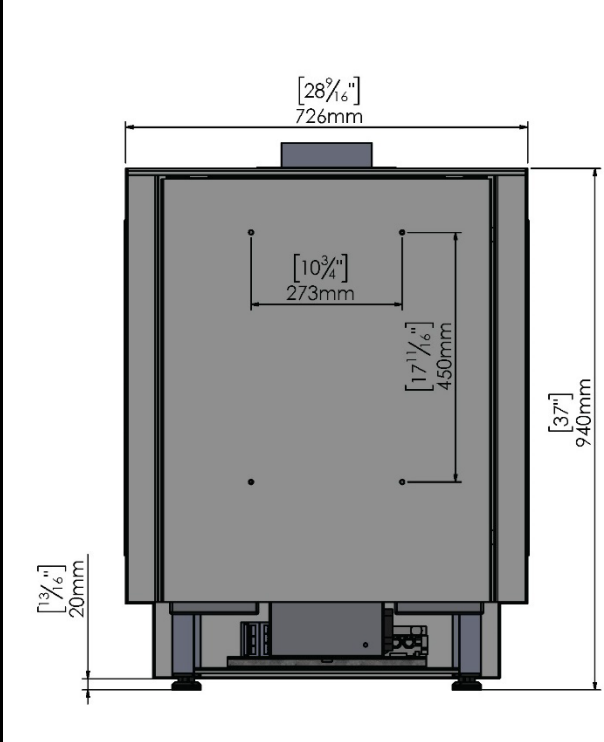
FLOOR-MOUNTED (legs, covered back)
