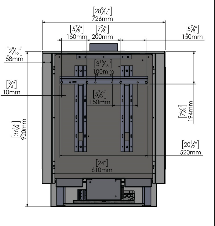
WALL-MOUNTED (no legs, exposed mounting attachments on back)
