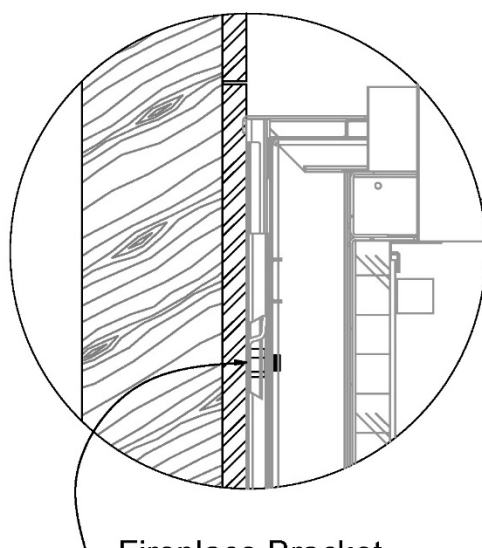
Fireplace Bracket Connection
