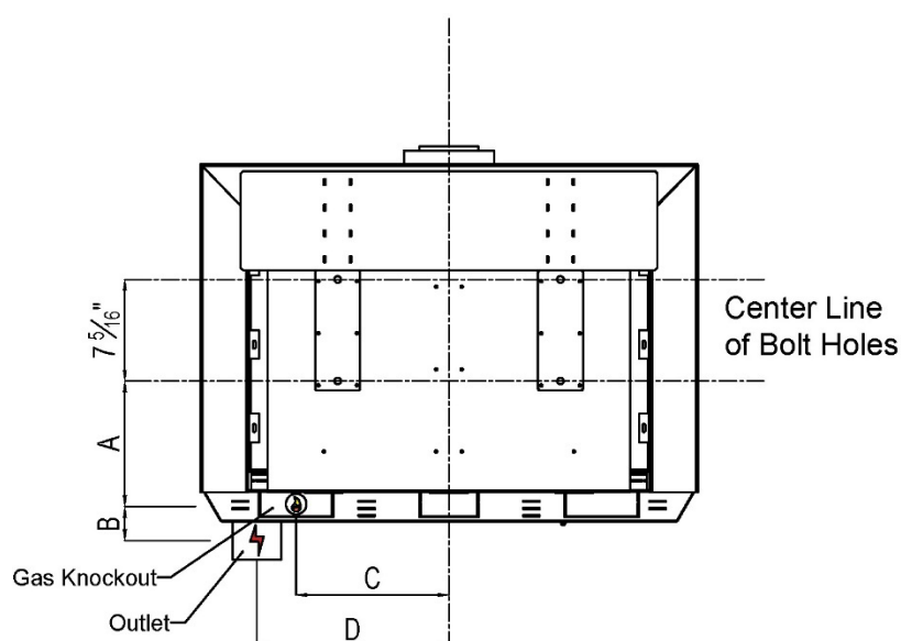
Back View
