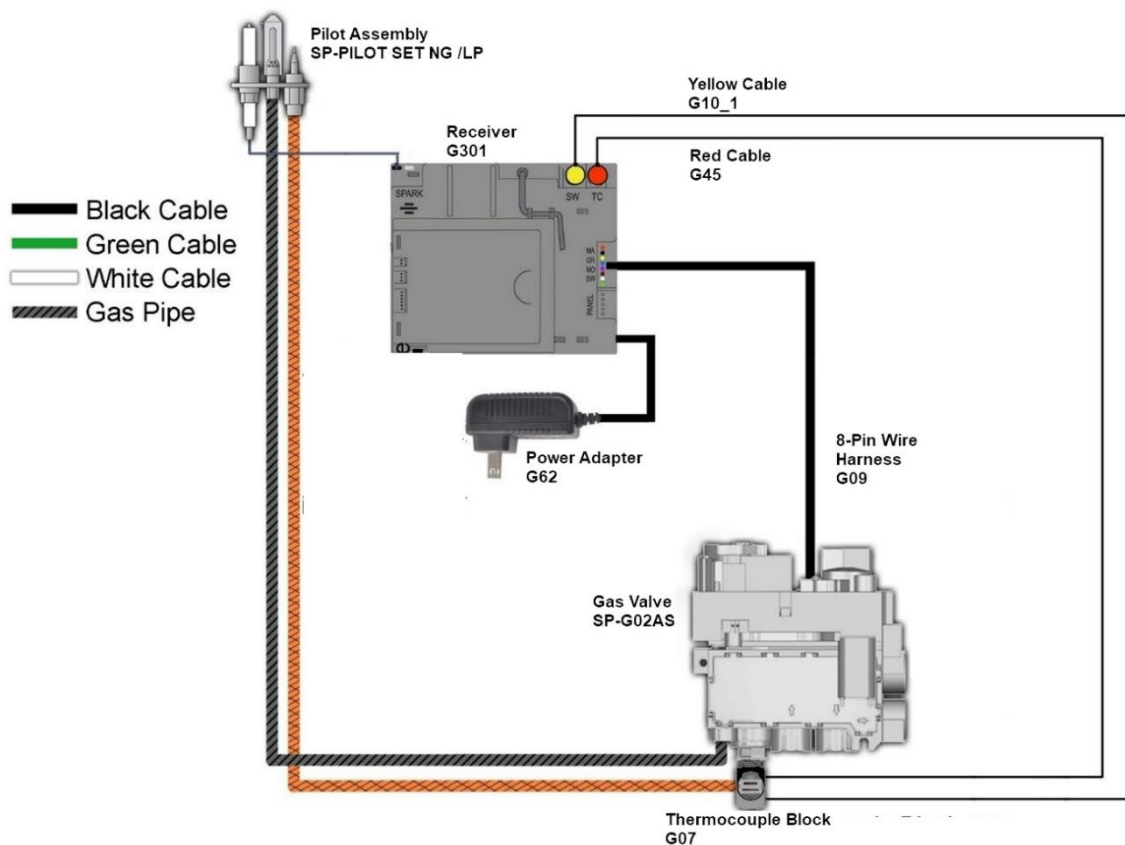
Wiring Diagram: Screened Series
