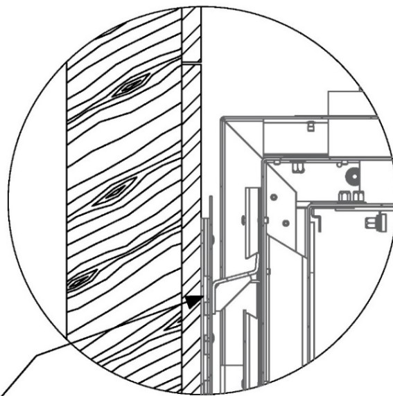
Fireplace-Bracket Connection
