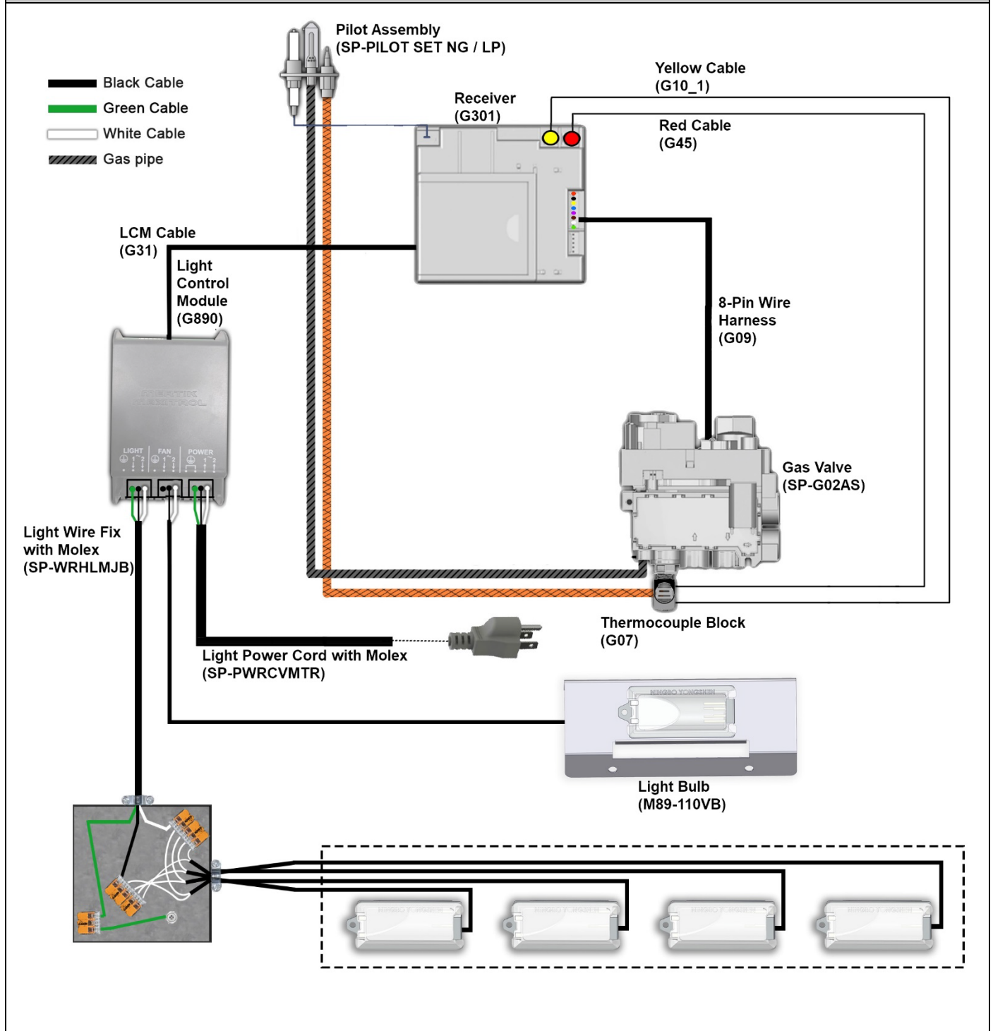
Wiring Diagram: Screen Fireplace with Interior Lighting
