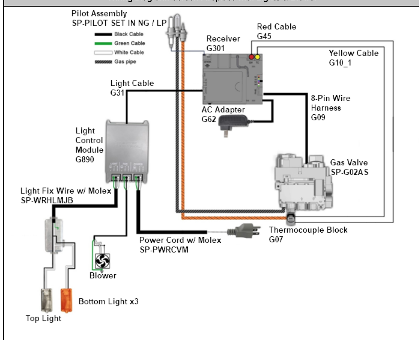
Wiring Diagram: Screen Fireplace with Lights & Blower
