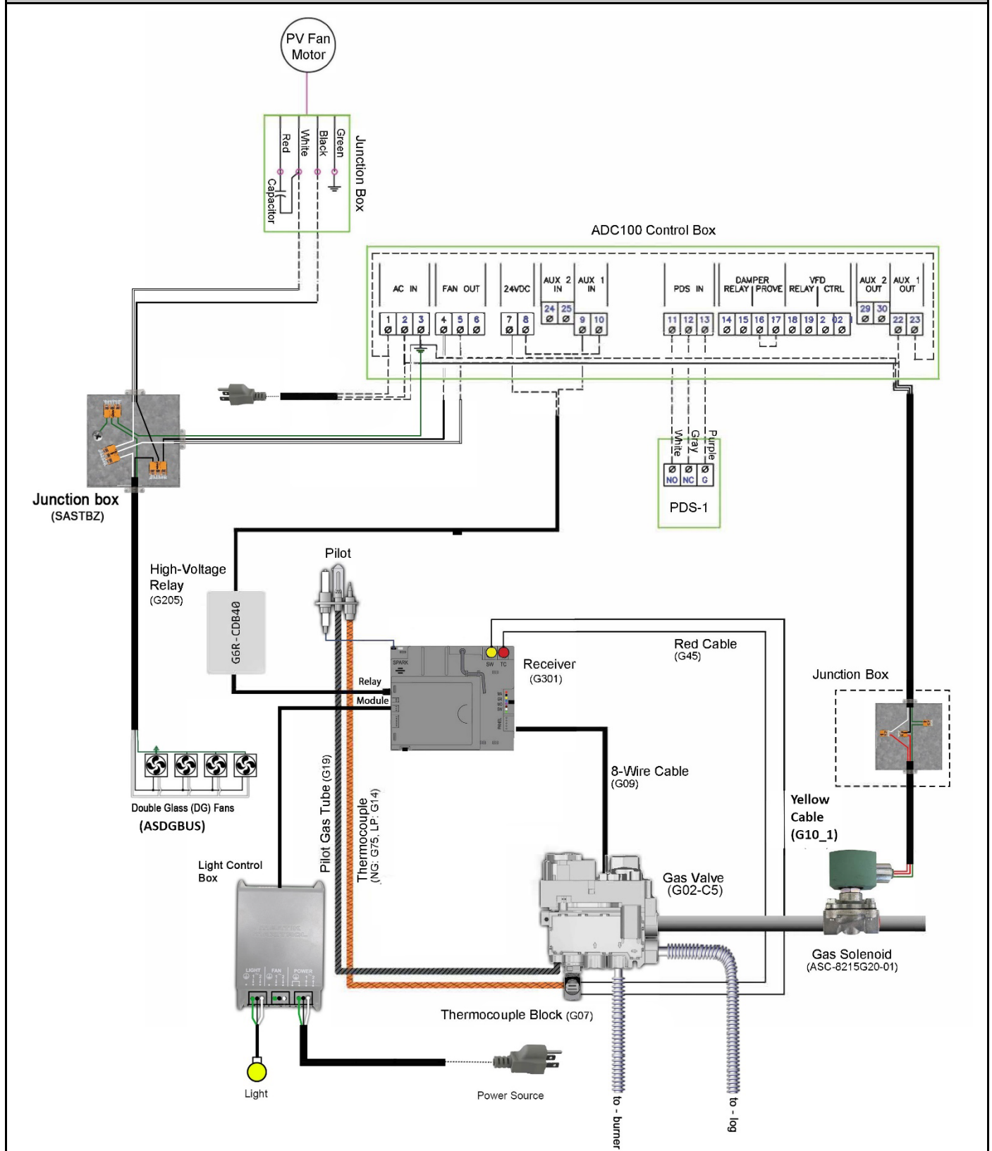
Wiring Diagram: Double Glass Fireplace with Interior Lighting and Enervex Power Vent
